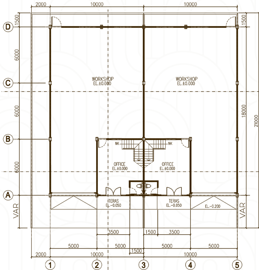
Denah Lantai 1
