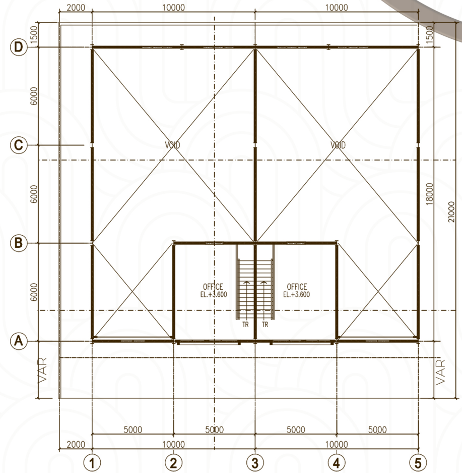
Denah Lantai 2
